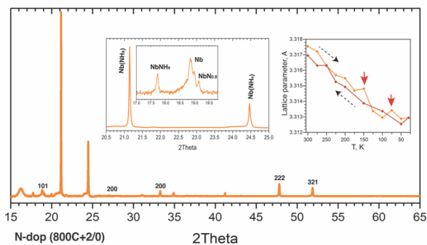
Figure 3: GIXRD patterns for the N-dop (800C+ 2/0) cutout recorded at 150 K. The main phases identified in this sample are Nb, and the solid solution \alpha -Nb(NH x ), accompanied by two minor phases, NbN 0.84 and NbNH x . Insets: (Right) Unit cell contraction and expansion during sample cooling and warming, respectively; (Left) reflections from \alpha -Nb(NH x ) phase.
