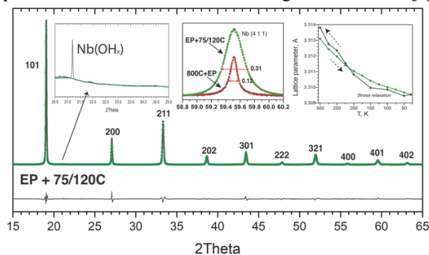
Figure 2: GIXRD pattern for the EP+75/120 °C cutout recorded at 150 K. This pattern is composed of by reflections from Nb (bcc cubic phase) and of the second cubic phase (fcc) ascribed to the presence of \alpha -Nb(OH) (Inset). The Nb phase shows a monotonous (regular) cell contraction and expansion during the cutout cooling and warming, respectively.
