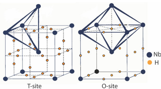
Figure 1: Interstitials tetrahedral (left) and octahedral (right) sites in the bcc Nb lattice.
