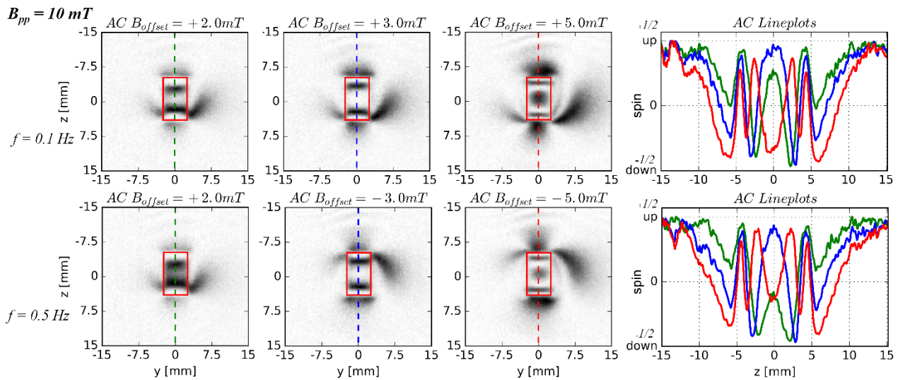
Figure 6: Radiographs of ac-field cooled sample. The field amplitude was always 10 mT peak to peak. The DC offset field and the frequency of the AC field were varied. The right graphs show the integrated spin phase change.
