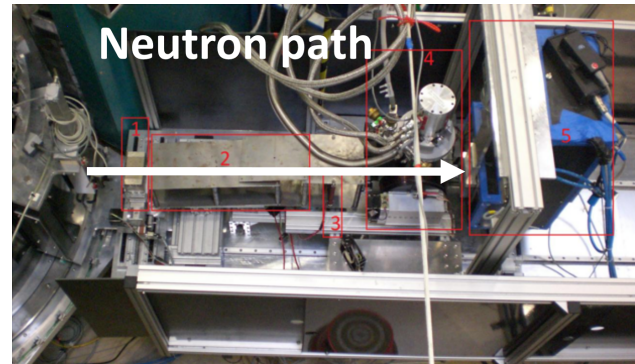
Figure 1: Photograph of the PONTON II set up from top: (1) polarizer, (2) guiding field, (3) spin flipper, (4) sample in cryostat and Helmholtz coils, and (5) neutron detector.
