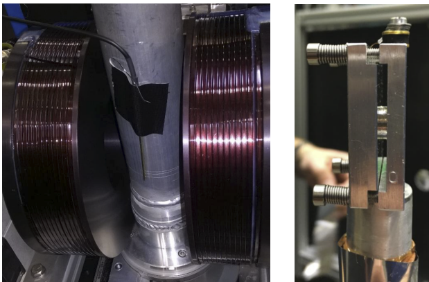
Figure 3: Left: Helmholtz coil used for field cooling of sample in cryostat. Maximum fields of 60 mT (85 mT for a short time) could be generated across the sample. Magnetic fields were measured with a Hall probe. Right: Holding frame and mounted Nb-sample.
