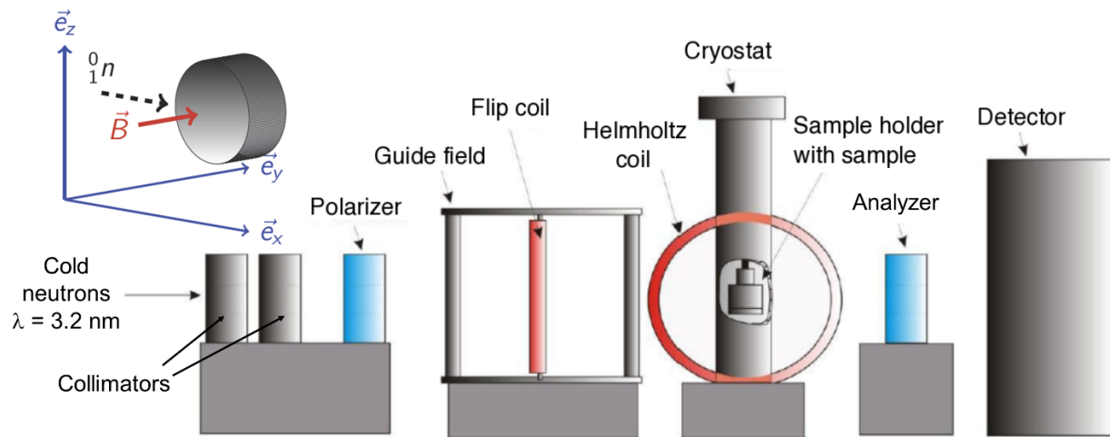
Figure 2: Setup of the PONT0 II experiment: Cold neutrons from the HZB reactor BER II reactor are collimated and spin polarized. The neutron trajectory leads through a guide field with the option to perform a spin-flip by a flip-coil, the sample inside a cryostat, and a spin analyzer, and it ends in the detector. The spin rotates in the magnetic field of a sample and hence typically approaches the spin analyzer in a non-parallel orientation. The angle of the final spin rotation depends on the magnetic field along the neutron path. Changes in the polarization reduce the transmission through the spin analyzer which leads to contrast information of the recorded images. The influence of the guide field has to be accounted for with calibration measurements. The inset shows the orientation of sample, neutron velocity and trapped magnetic field, here: 0^\circ position).
