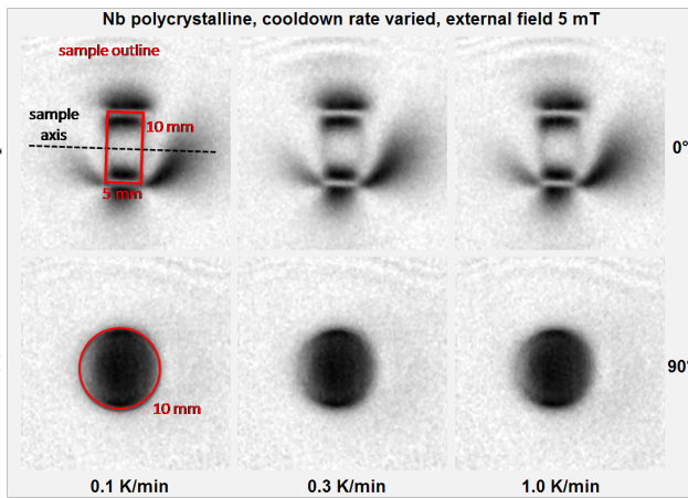
Figure 4: Cooling in external magnetic field of 5 mT at varying rates. The neutron beam is always perpendicular to the paper plane. The sample outline and dimensions are indicated in red. Upper row: 0° sample orientation, lower row: 90° sample orientation.
