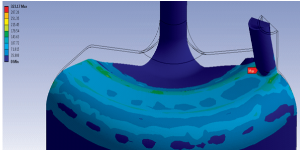
Figure 2: von-Mises stress on the end cap under 1 atm external vacuum load.
