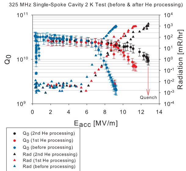
Figure 4: 325 MHz single-spoke cavity test results before and after helium processing.
