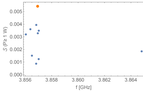
Figure 8: (Cumulative) probability S that loss is greater than 1 W, for the different modes. The orange dot indicates the strongest mode, i.e. the mode with the largest loss factor \kappa .
