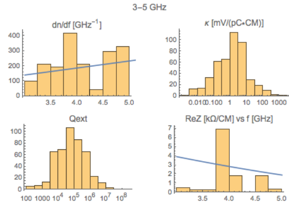
Figure 4: Statistics of modes: density of modes, dn/df [GHz ^{-1} ] vs. f [GHz] (top left), histogram of loss factors \kappa [mV/(pC*CM)] (top right), histogram of Q 's (bottom left), and \text{Re}(Z) [kΩ/CM] vs. f [GHz]. Lines gives expected density of modes and \text{Re}(Z) .
