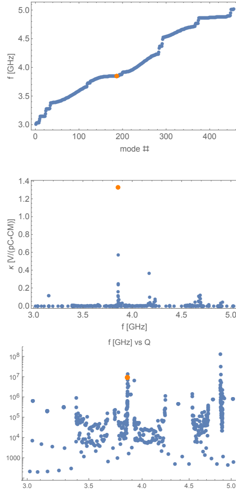
Figure 3: Mode properties: frequencies f_m (top), loss factors \kappa_m vs. f_m (middle), and quality factors Q_m vs. f_m in [GHz] (bottom). The strongest mode is shown in orange.
