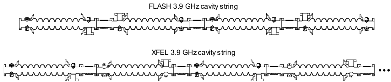
Figure 4: Possible cavity arrangements for installing the power couplers alternately opposite to each other.
