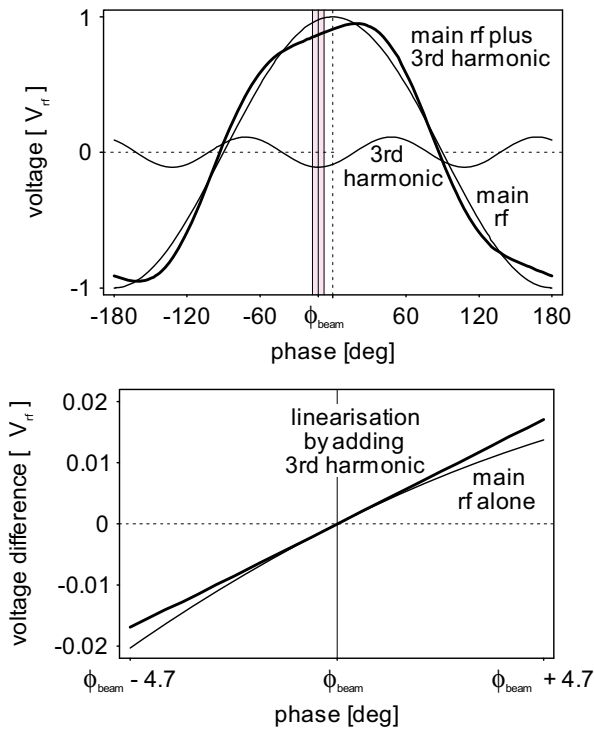
Figure 2: Linearisation of the voltage chirp seen by the beam adding a third harmonic rf system with decelerating phase.
