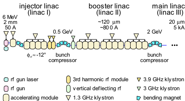
Figure 1: Sketch of the first part of the European XFEL accelerator where the bunch compression takes place.
