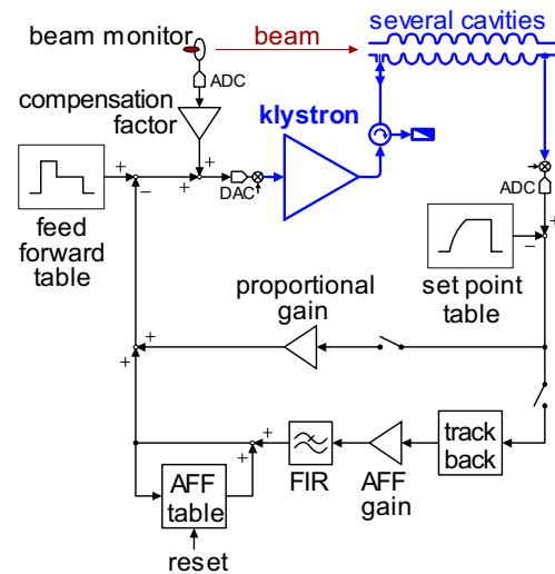
Figure 7: Potential scheme of the digital third harmonic rf control (black) surrounding the high power rf (blue). DACs in front of the vector modulator ( \otimes ) and ADCs after down converters ( \otimes ) are part of the digital electronics.
