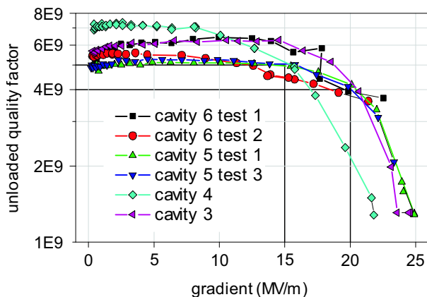
Figure 5: Vertical test results of 3.9 GHz cavities produced for the FLASH 3rd harmonic module.
