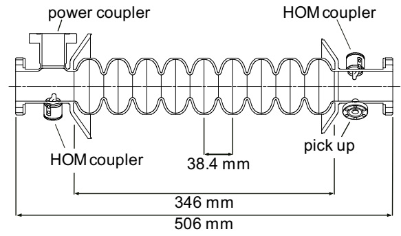
Figure 3: Side view of a nine cell 3.9 GHz cavity with the main power coupler, the pick up probe, and two higher order mode (HOM) couplers.
