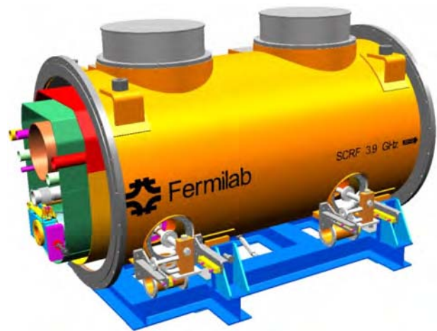
Figure 6: FLASH 3rd harmonic module manufactured at Fermilab. Experience gained with this module will influence the XFEL 3rd harmonic module design.
