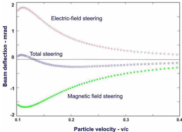
Figure 3: Steering of a proton beam for a single 115 MHz QWR cavity operating at E_{acc} = 5 MV/m, and a phase of -30 degrees.
