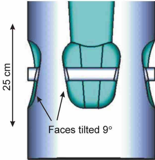
Figure 2: Detail of the beam-interaction region of the 115 MHz QWR cavity
