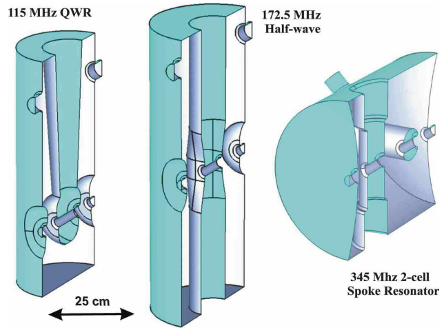
Figure 1: Sections of the niobium shell for three SC cavities covering a velocity range of 0.11 < \beta < 0.6
