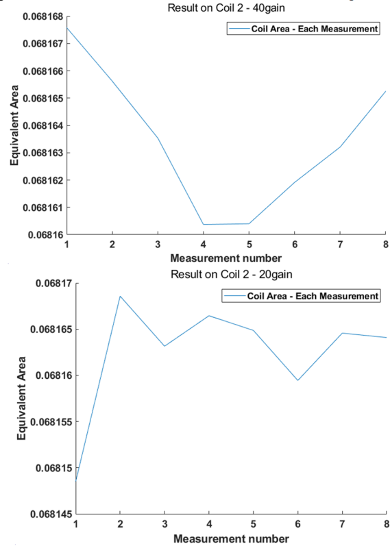
Figure 2: Calculated result of equivalent area of coil 2.
