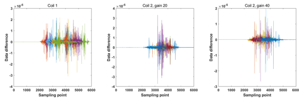
Figure 3: Difference in integral's gradient and voltage data.
