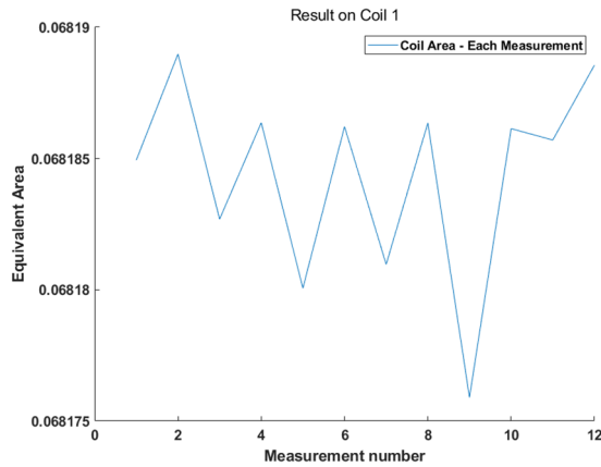
Figure 4: Calculated result of equivalent area of coil 1.
