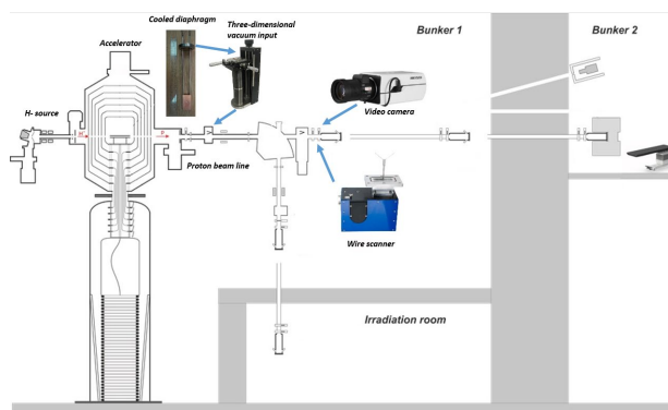
Figure 1: Experimental setup.
