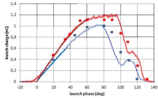
Figure 7: RF lunch phase influence. E_{\text{cathode,max}} = 62 MV/m (red curve) and E_{\text{cathode,max}} = 47.6 MV/m (blue curve). Crosses mark the SUMA calculation results.
