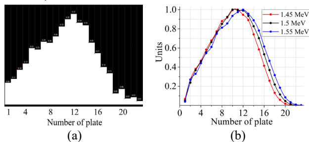
Figure 9: Experimental (a) and calculated (b) distribution of charge over the plates (1.5 MeV).
