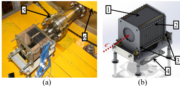
Figure 8: Experiment scheme (a) and measuring assembly (b): 1 – aluminum plates; 2 – current pickups; 3 – retention flanges; 4 – fan; 5 – output device; 6 – accelerating cavity.
