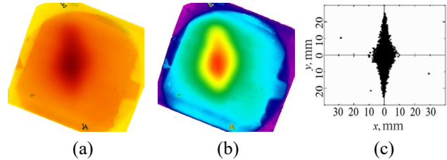
Figure 6: Beam image (a), reconstructed gradient image (b) and calculated transverse beam profile (c).
