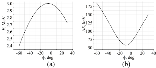
Figure 4: Average electron energy (a) and energy spread in a bunch (b) at various injection phases (two passes).
