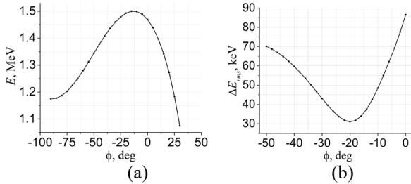
Figure 3: Average electron energy (a) and energy spread in a bunch (b) at various injection phases (single pass).
