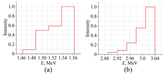
Figure 11: Reconstructed electron energy spectrum after one pass (a) and two (b) passes.
