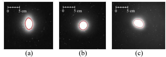
Figure 7: Scintillator glow image: 1.5 MeV with no quadrupole lens (a), 1.5 MeV with quadrupole lens (b) and 3 MeV (c).
