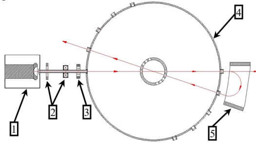
Figure. 2: Acceleration scheme: 1 – RF injector; 2 – focusing solenoids; 3 – quadrupole lens; 4 – accelerating cavity; 5 – bending magnet.
