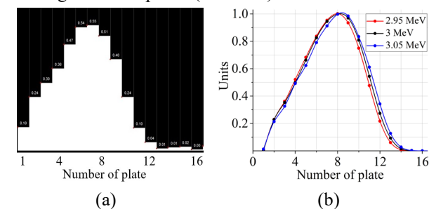
Figure 10: Experimental (a) and calculated (b) distribution of charge over the plates (3 MeV).
