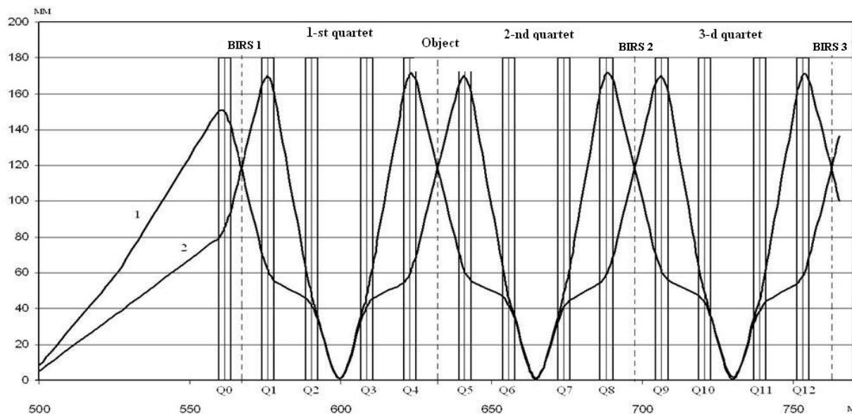
Figure 2: The structure of the quartets (shown beam envelopes in the horizontal (1) and vertical (2), Q1-Q12 quartet lenses).
