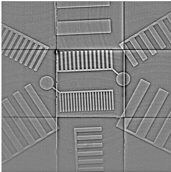
Figure 6: Proton radiography image of the object in microscope mode.
