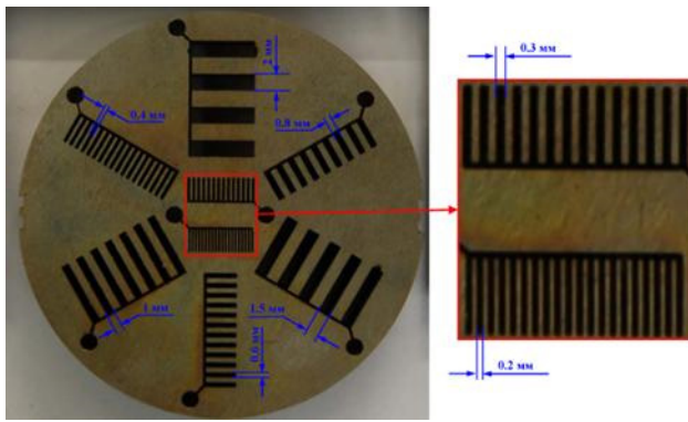
Figure 5: The radiography object.
