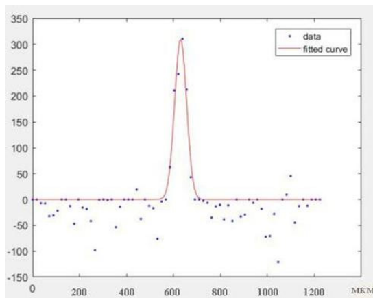
Figure 7: Measured blur function in the horizontal plane.
