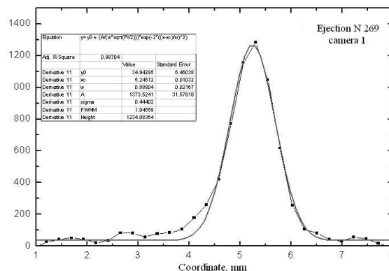
Figure 4: Measured blur function of the boundary for object with a thickness of 350 g/cm 2 .
