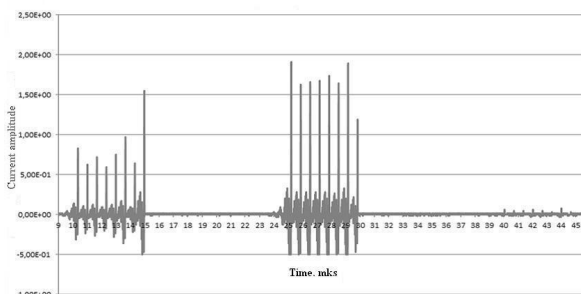
Figure 3: Current signal of the extracted beam in the FRE mode.
