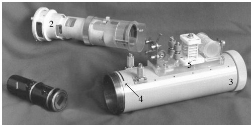
Figure 2: Dissector LI-602 used in BINP
