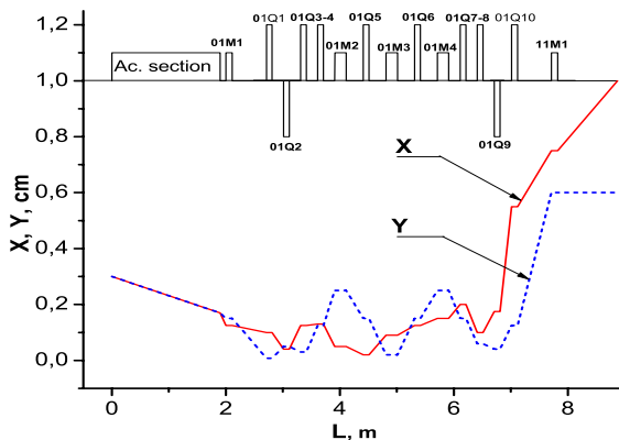
Figure 3. The beam envelope for injection energy 28 MeV.
