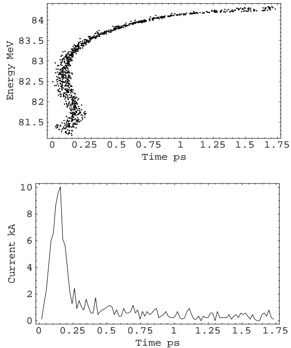
Figure 3: PARMELA simulation of compressed bunch exiting chicane.
