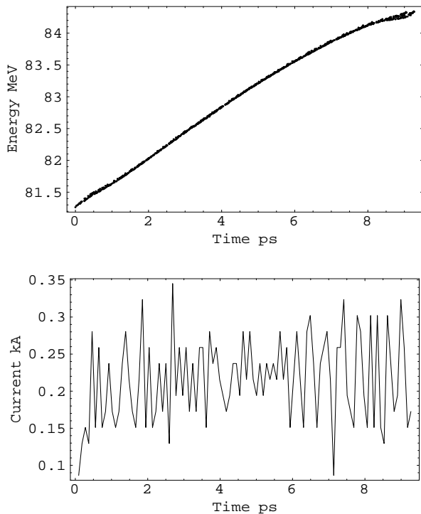
Figure 2: PARMELA simulation of energy-chirped beam entering chicane.
