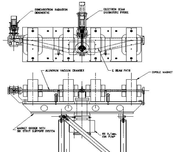
Figure 1: Magnetic chicane.
