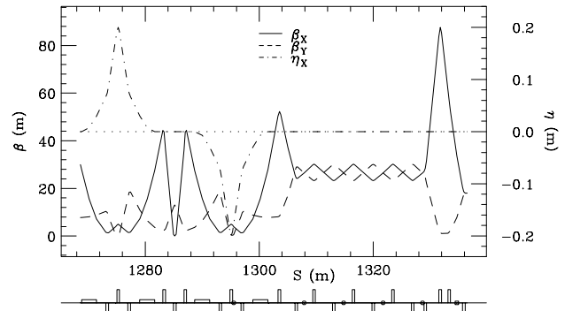
Figure 4. DL2 Beam Transport Line. Note the wire scanners for beam emittance and energy measurement in the magnet schematic.
