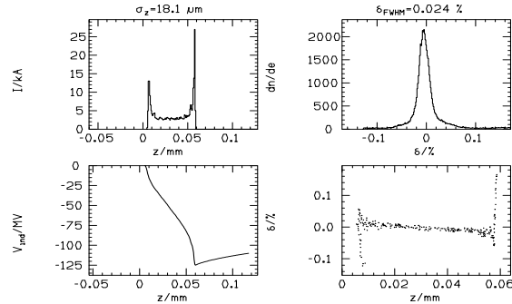
Figure 6. Longitudinal Bunch Distributions to Undulator at 15 GeV. The plot shows z-distribution (top left), energy distribution (top right), longitudinal wakefield (bottom left) and energy-z correlation (bottom right).
