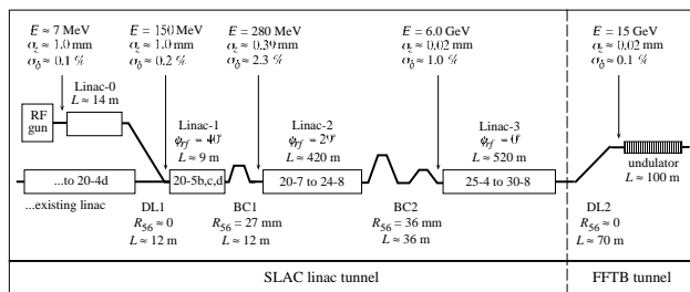
Figure 1. LCLS Linac Schematic
