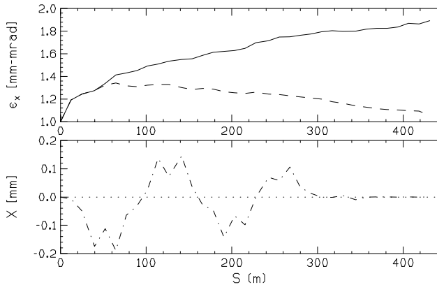
Figure 3. Emittance Bumps in L2. The upper plot shows emittance dilution without (solid) and with (dashed) emittance bumps. The lower plot shows a typical horizontal orbit distortion due to the bump.
