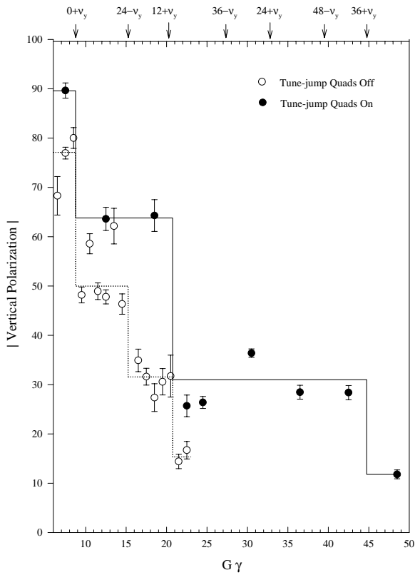
Figure 1: Results of AGS 5% partial snake test. The measured absolute value of the vertical polarization at G\gamma = n + \frac{1}{2} up to G\gamma = 48.5 . The open circles are the results without the tune-jump quadrupoles and the solid points are the results with the tune-jump quadrupoles.
