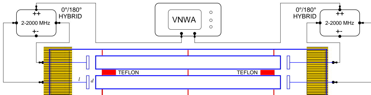
Figure 1: Experimental setup: a vector network analyser (VNWA) is used in conjunction with two hybrids, yielding either even (++) or odd (+-) mode excitation for a 1 m long cylindrical cavity with two inner conductors, held by 3 teflon supports. The near degeneracy of even and odd modes is removed by two teflon splitters placed between the inner conductors.
