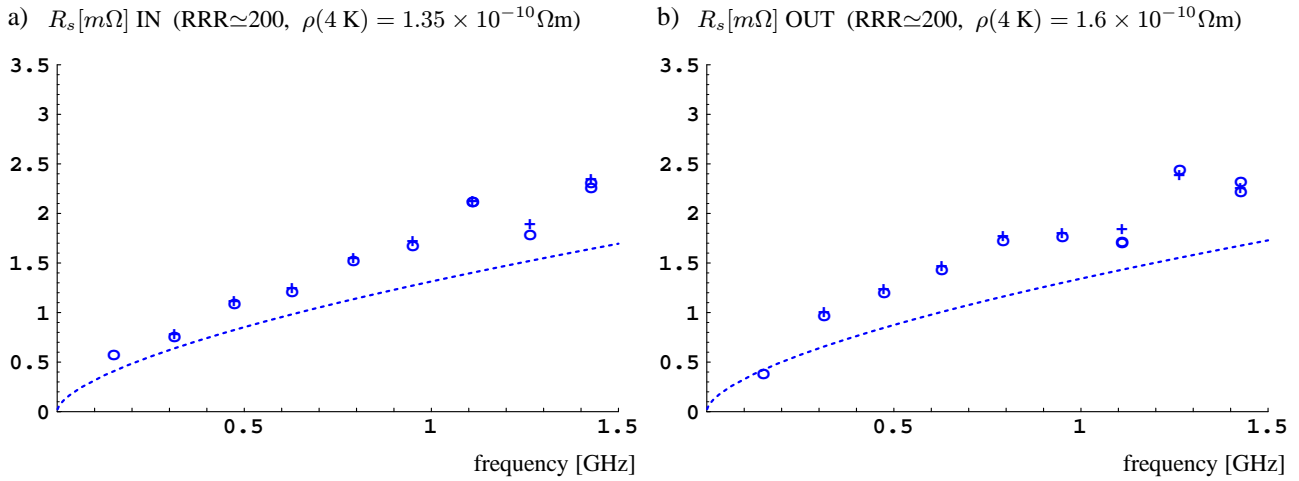
Figure 3: Surface resistance measured with shorter coupling networks at 4 K (“o”) and at 20 K (“+”) for the inner conductors (a) and the outer tube (b), both thermally treated at 350° C and having a measured dc RRR \simeq 200, compared to the predictions in the anomalous regime (dashed lines). The corresponding data at room temperature (not shown in the figure) is best fitted assuming a resistivity \rho(300\text{ K}) = 2.7 \times 10^{-8}\Omega\text{m} for the inner conductors and \rho(300\text{ K}) = 3.2 \times 10^{-8}\Omega\text{m} for the outer tube. The slightly higher resistivity attributed to the inner conductors may be due to small scratches in their copper coating, caused by the sliding teflon supports repeatedly mounted during previous measurements.
