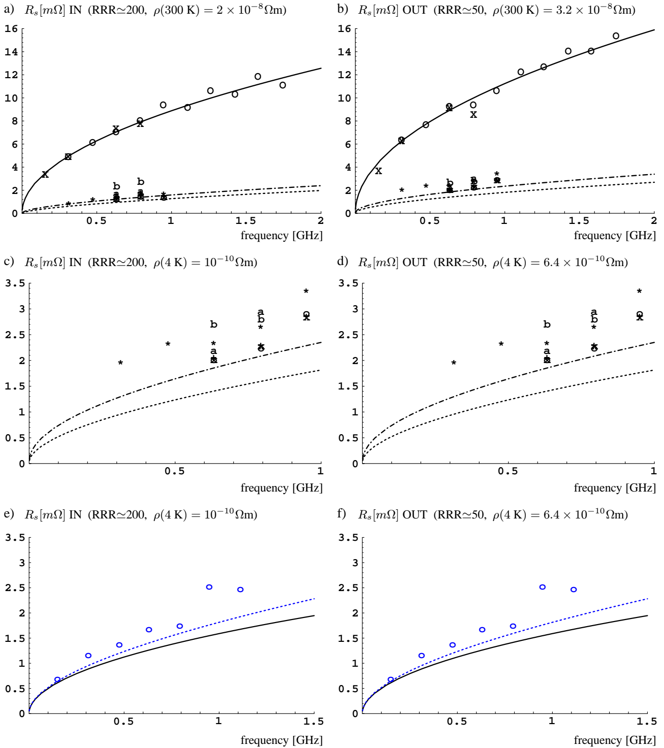
Figure 2: Surface resistance measured for the thermally treated inner conductors (a, c, e) having a dc RRR \simeq 200, and for the outer tube (b, d, f) with no thermal treatment and a dc RRR \simeq 50, compared to the predictions in the classic (solid line) and anomalous regime (dot-dashed lines: 40 K, dashed lines: 4 K). Figures (a) and (b) show data measured at room temperature, either before (“X”) or after cryogenic measurements using shorter coupling networks (“O”), at 40 K, either before (“b”) or after (“a”) injection of He gas during cool down (leading to a sudden thermalisation of the inner conductors, otherwise thermally insulated) or with external heating (“*”), at 20 K (“+”), at 10 K (“x”) and at 4 K (“o”). Some measurements at 40 K have a large temperature spread from top to bottom of the outer tube. The data at room temperature is best fitted assuming a resistivity \rho(300\text{ K}) = 2 \times 10^{-8}\Omega\text{m} for the inner conductors and \rho(300\text{ K}) = 3.2 \times 10^{-8}\Omega\text{m} for the outer tube. Figures (c) and (d) are a magnification of (a) and (b), respectively, showing only measurements at cryogenic temperatures. The data in (e) and (f) has been obtained at 4 K with shorter coupling networks, to allow measurements in a wider frequency range: data above 1.2 GHz, however, has been discarded due to strong or badly corrected coupling.
