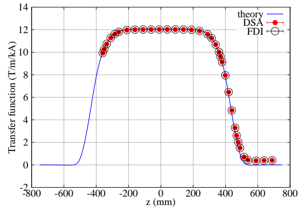
Figure 2: Axial dependence of main field ( B_2 ) transfer function measured at \sim 70 K with I = 30 A using the 100 mm coil.
