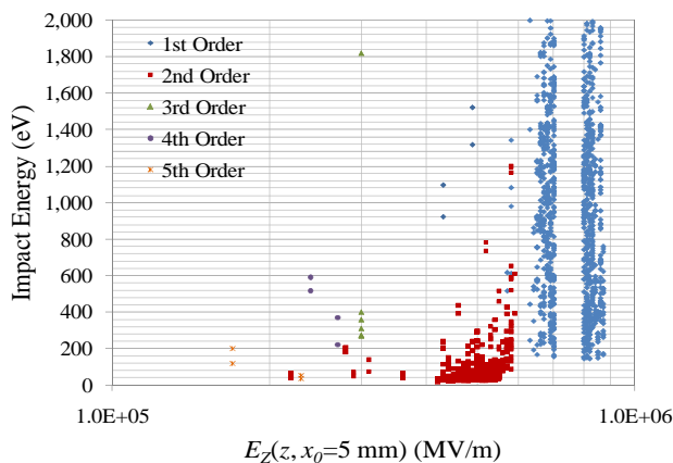
Figure 5: Impact energies for field gradient range of 10 kV/m to 1 MV/m for area (A).
