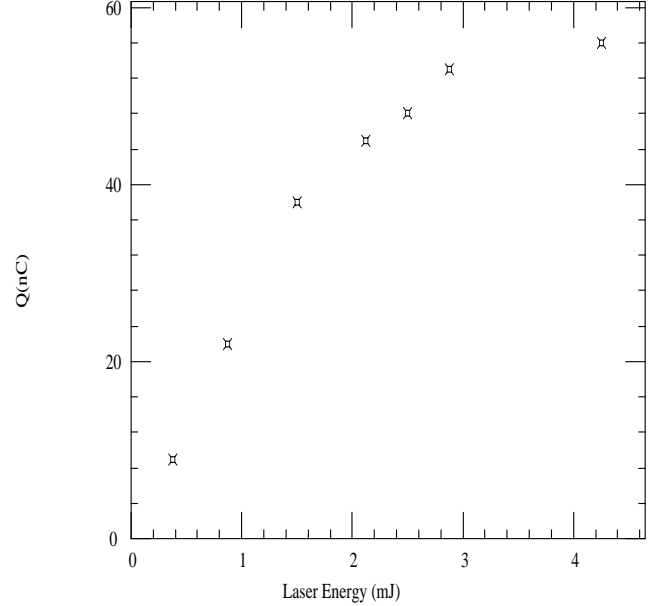
Figure 3. Measured beam intensity as a function of laser energy. (Magnesium photocathode).
