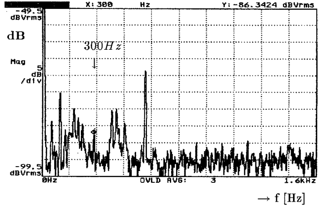
Figure 2. The horizontal phase-locked-loop spectrum at 820 GeV with an additional tune modulation of 300 Hz and \triangle Q \approx 10^{-4} . The additional tune modulation compensates the 300 Hz line of the original phase-locked-loop spectrum.
