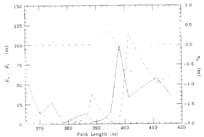
Figure 5b. Betatron envelope functions in staircase recombining.
