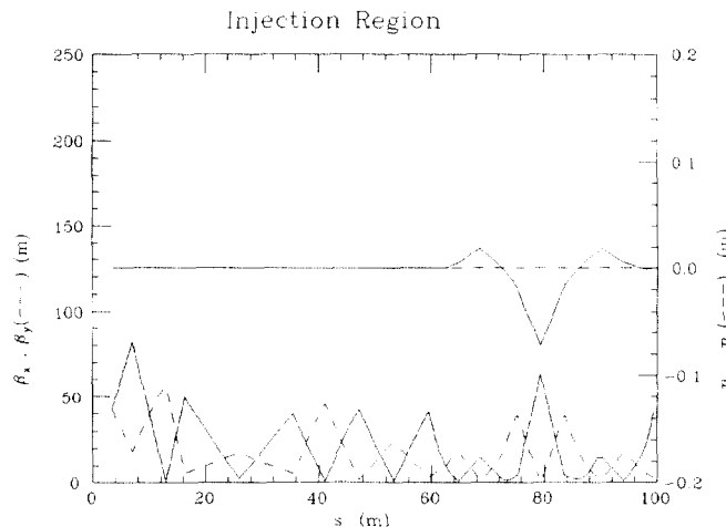
Figure 2. Betatron parameters for injector and chicane.
