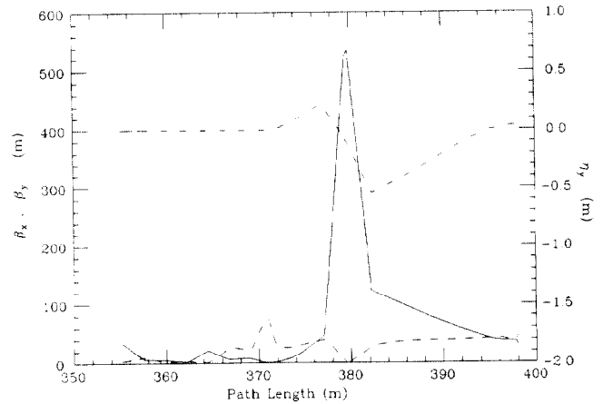
Figure 5a. Betatron envelope functions in one-step recombining.
