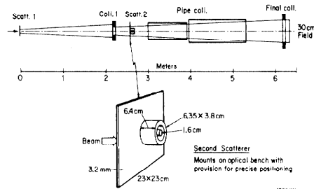
Fig. 5. Beam flattening system used at the LBL 184" cyclotron and the Bevalac. Occluding rings block out portions of the Gaussian-shaped beam. Scattering plus drift length combine to produce a very uniform distribution at the site of the patient.
