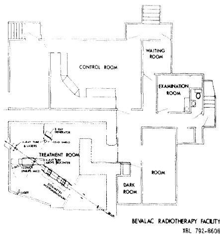
Fig. 1. Schematic layout of the Radiotherapy facility showing the treatment room, and ancillary areas. The area marked "room" houses the technician's control station, viewing boxes and a discussion area for physicians and physicists.
