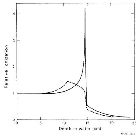
Fig. 4. Range-energy curves measured for a typical heavy ion beam at the Bevalac; the unmodified curve (solid line) showing characteristically sharp stopping point, and the spread-out curve (dashed line) resulting from passage through the ridge filter. The ionization beyond the stopping point in both curves is due to nuclear projectile fragments, which have longer ranges than the primary beam.
