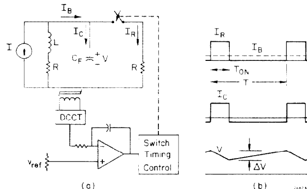
FIG. 2--(a) Elementary chopper and control circuit; (b) voltage and current waveforms.
