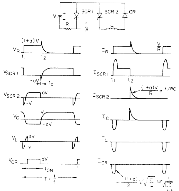
FIG. 4--Jones chopper.
