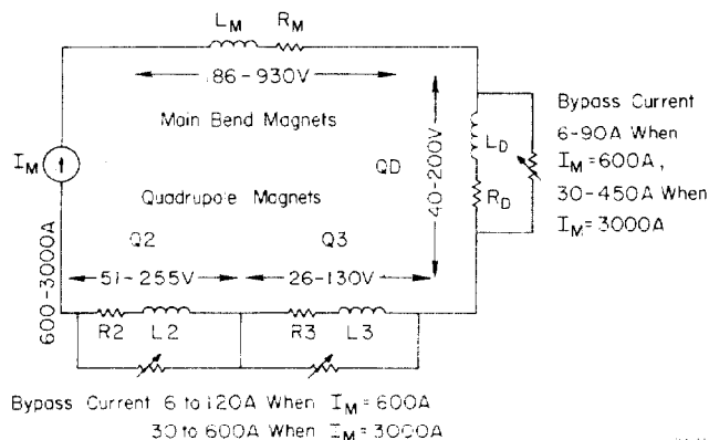
FIG. 1--Magnet current bypass shunts for SPEAR.
