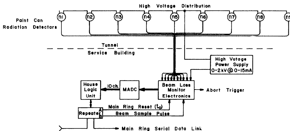
Fig. 1. A Main Ring Service Building Beam Loss Monitor Subsystem configuration. Paint can detectors are identified by tunnel survey marks n1 through n9, where n specifies service buildings 1 through 4 per Main Ring sector, n1 detectors exist only for n = 1,2 service buildings. These configurations are identically repeated in Main Ring Sectors A through F.
