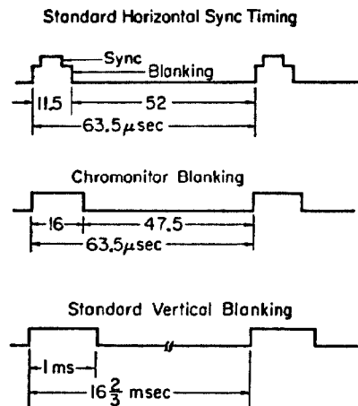
Figure 2. TV synchronizing signals for horizontal and vertical sweep in the NTSC raster scan system. Modification for the Chromonitor is shown in the center.
