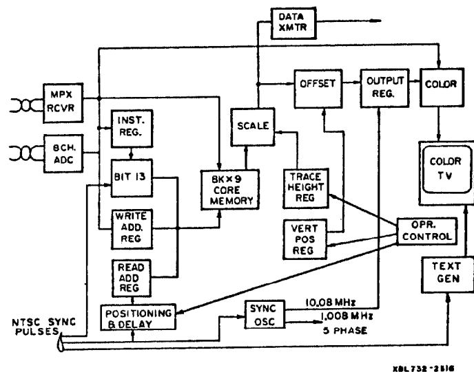
Figure 1. Simplified block diagram of the Chromonitor. Implementation for 16 traces requires one hundred 5" x 5" circuit cards.
