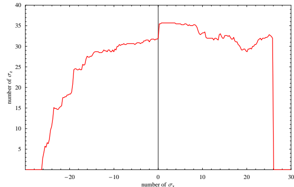
Figure 1: Dynamic aperture for 1000 turns without a defect in the dipoles. The horizontal and vertical emittances are taken equal to 0.22 \pi mm.mrad
