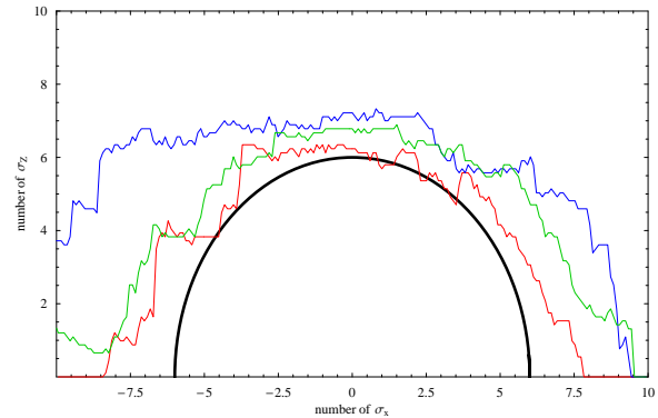
Figure 6: Dynamic aperture at 1000 turns for the working point A for different multipole defect values after optimization (in red for the reference values given in Table 1, in green for the reference values divided by 1.5 and in blue for divided by 2)
