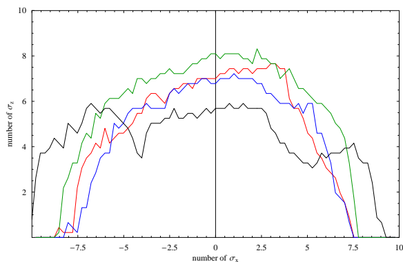
Figure 2: Dynamic aperture for 1000 turns for the same structure as in [1]. In red, n = 5 component, in blue n = 7 component and in green n = 9 component, in black with every systematic multipolar component
