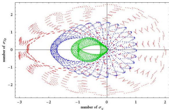
Figure 5: Representation in the horizontal normalized plane of the successive positions of an ion of the stored beam at \delta = 0 and with an initial amplitude ( x = 0, z = 5\sqrt{\beta_z\epsilon_z} ) for different working points after optimization (in red for the working point A , in blue for B and in green for C )
