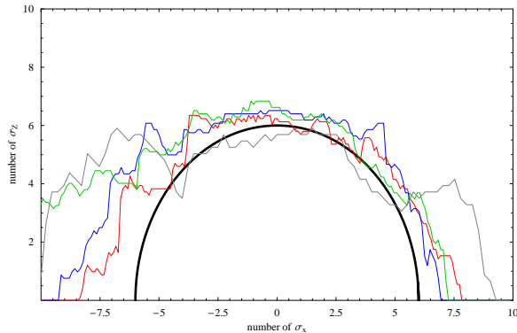
Figure 4: Dynamic aperture at 1000 turns for different working points after optimization (in gray for A before optimization, in red after, in blue for B and in green for C )
