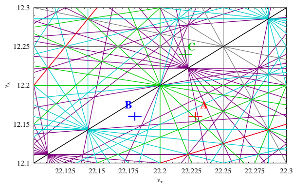
Figure 3: Tune diagram. In black, 2^{nd} order resonances, in red 3^{rd} order resonances, in gray 4^{th} order resonances, in green 5^{th} order resonances, in cyan 7^{th} order resonances and in purple 9^{th} order resonances. The different working points are represented by crosses on the diagram
