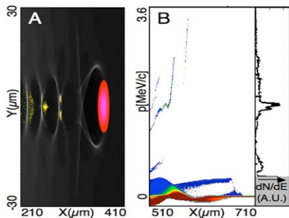
Figure 3: Particle simulations show that wave breaking on a plasma density downramp produces MeV electron bunches. At the location where the pulselength is near resonant with the density (A), the laser pulse (red) excites a large wake (density, grayscale). Variation of \lambda_p (visible in the density) due to the ramp decreases wake velocity and trapping threshold, leading to trapping of an electron bunch (particles with E > 0.5 MeV/c, yellow). The bunch phase space (B, red=maximum) shows a narrow momentum spread bunch at 1.5 MeV/c. The lineout at the right side of the phase space shows the momentum spectrum.
