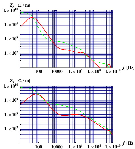
Figure 1: Vertical impedance at injection (top) and top energy after the squeeze (bottom). The full (red) line denotes the real part of the impedance, while the dashed (green) line is for the imaginary part.
