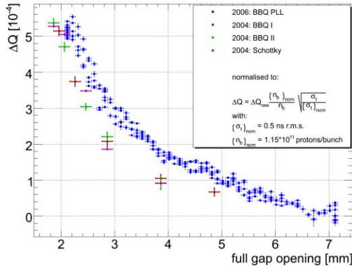
Figure 7: Measured coherent tune shift in the SPS in 2006 compared to 2004 vs. collimator full gap.
