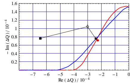
Figure 4: Stability limits: (Filled square) nominal secondary collimator resistivity ( 10^{-5} \Omega m ), (unfilled diamond) secondary collimator resistivity of 1.7 \cdot 10^{-8} \Omega m (copper), (filled star) secondary collimator resistivity of 10^{-10} \Omega m , (red dot) without secondary collimators.
