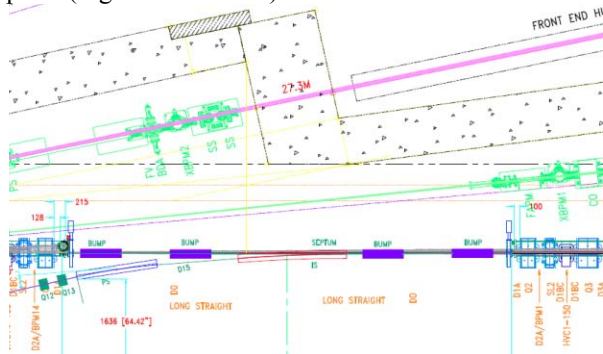
Fig. 4: Injection straight section layout
