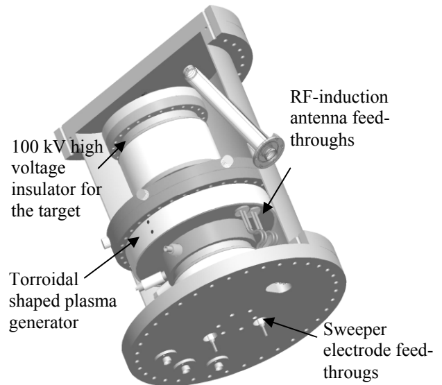
Figure 4: Cut-out drawing of the fast pulsing point neutron generator. The device is ~100 cm tall and ~50 cm in diameter.
