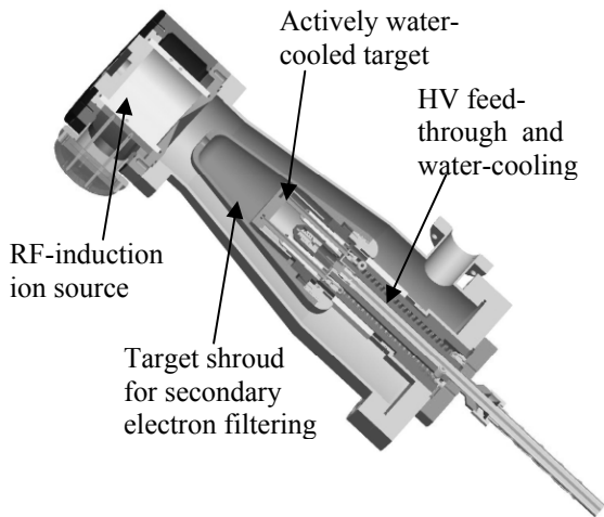
Figure 1: Fully high voltage shielded and grounded neutron generator design for medium neutron yield.
