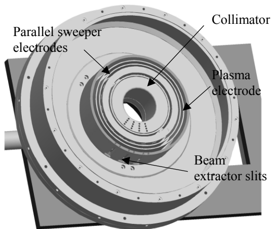
Figure 7. Cut-out view of the beam sweeper prototype. The prototype is built to test and verify the ion beam simulation results in a realistic geometry. The beam pulsing speed and the current will be measured from one extracted beamlet, using a 50 Ohm impedance matched faraday-cup placed the target position in the middle of the device.
