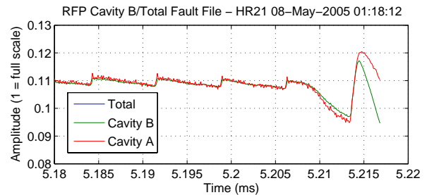
Figure 2: HER 12-1 Gap Voltage at abort.
