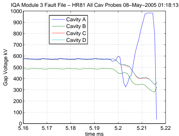
Figure 4: HER 8-1 Cavity A arc.
