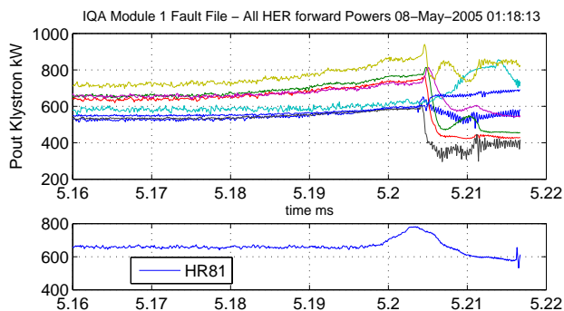
Figure 3: All Klystron forward powers in HER.
