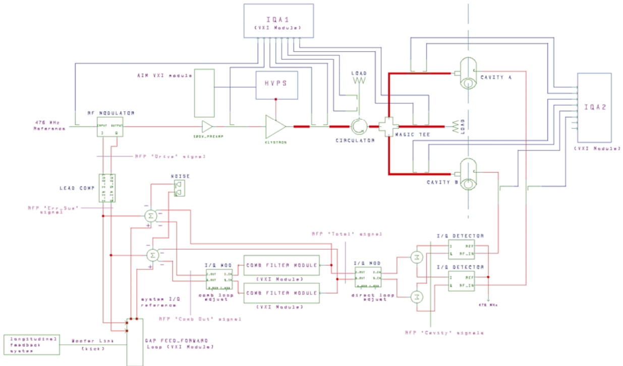
Figure 1: PEP-II LLRF signal diagnostic block diagram.
