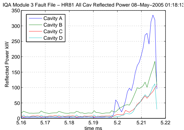
Figure 5: HER 8-1 Reflected Power.
