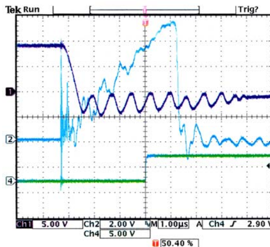
Figure 4: Opening switch arc response. Top trace: load voltage. Middle trace: load current. Bottom trace: switch control signal. The opening switch response time is 1.3 \mu s after threshold crossing.
