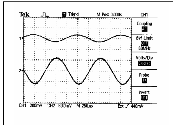
Figure 7: Linear voltage control. Top: 4 kV sinusoid in response to a signal generator sine wave input.
