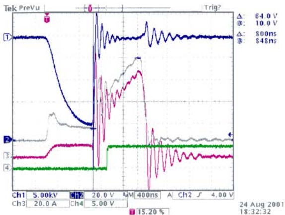
Figure 2: 50 kV klystron arc and opening switch response. Trace 1 – cathode voltage; Trace 2 – switch current; Trace 3 – cathode current; Trace 4 – switch controls signal. Power is removed at ~600 ns after arc onset. Total arc energy is << 1 J.
