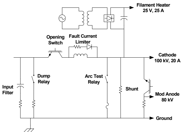
Figure 3: Solid-state switch schematic for the 100 kV, 100 A CW transmitter opening switch at the Advanced Photon Source.
