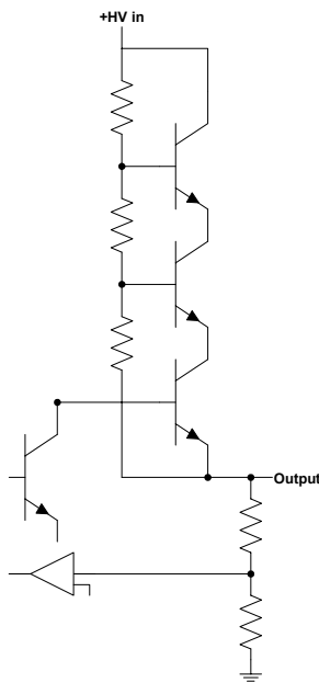
Figure 6: Simplified schematic of linear regulator.
