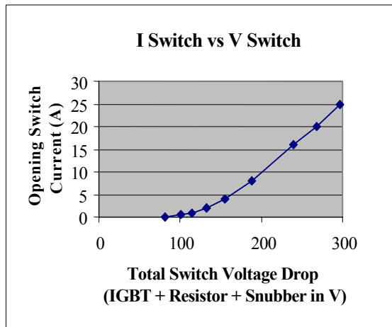
Figure 5: Voltage drop as a function of current in the 100 kV ANL switch. Efficiency at full current is 99.7%.
