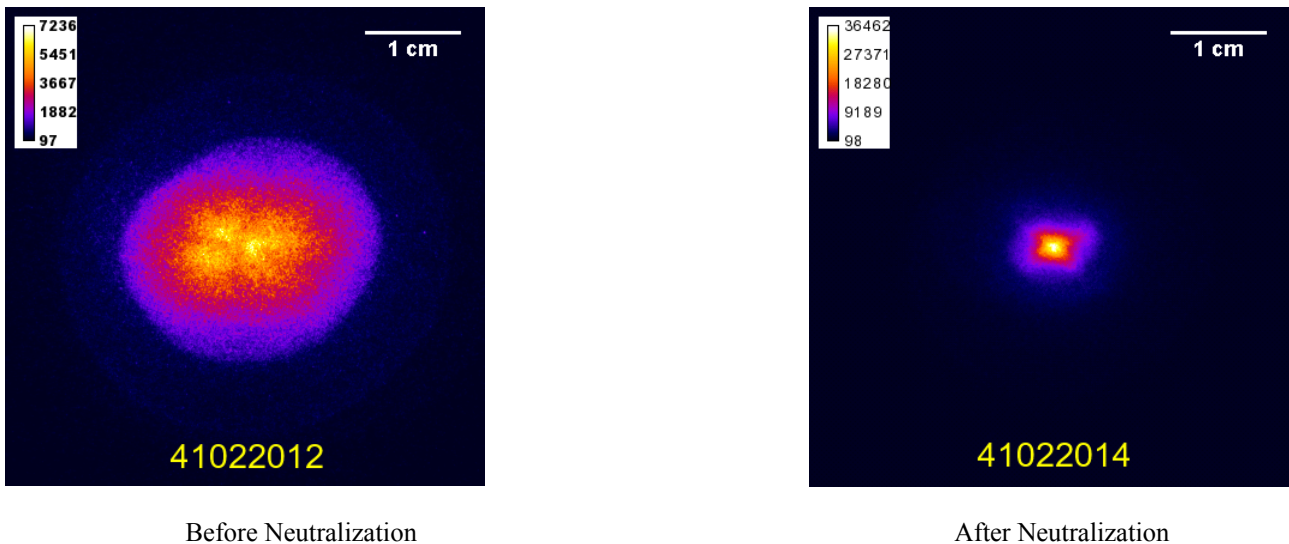
Figure 4: Images of the beam spot size before and after neutralization.
