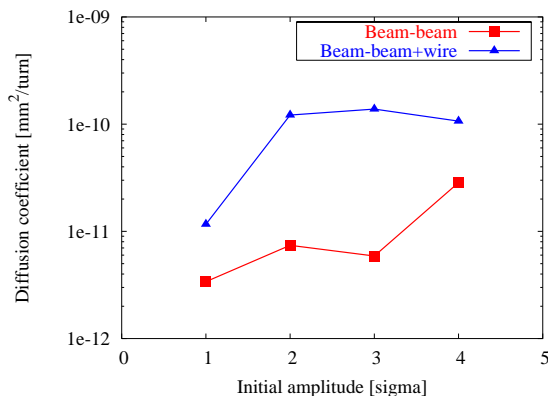
Figure 6: Horizontal diffusion coefficients of the two nearest parasitics to B0, without wire and with wire placed to cancel the average kick felt by the anti-proton beam.
