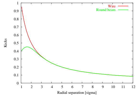
Figure 1: Kicks from a round beam compared to the kick of a round wire as a function of distance. At distances larger than 3\sigma , the kicks agree to better than 1%.
