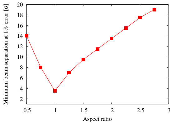
Figure 3: Minimum beam separation required to match a 1/r field as a function of the aspect ratio of an elliptical beam.
