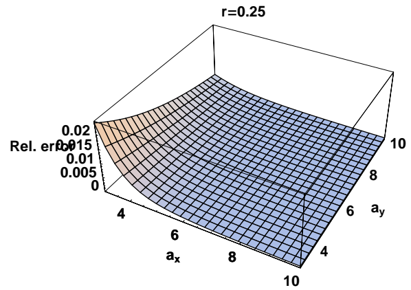
Figure 4: The relative error between an elliptical wire and elliptic beam-beam kicks as a function of amplitude outside the core for small aspect ratio.
