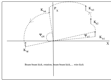
Figure 5: Phase space point following several beam-beam kicks, phase rotation between these kicks and ending up at a wire.
