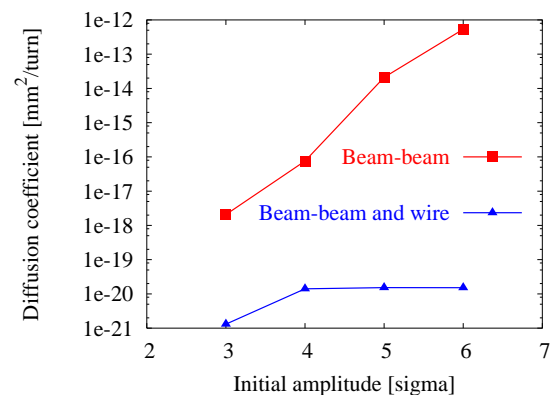
Figure 2: Diffusion coefficients for the local correction of a parasitic interaction where the beams are round and the separation approximately 10\sigma .
