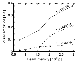
Figure 5: Fourier amplitude of three different frequencies versus beam intensity as measured with the microphone.
