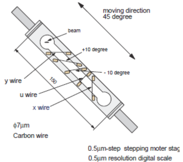
Figure 8: Carbon wire mount in the wire scanner.
