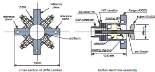
Figure 6: DR button BPM.
