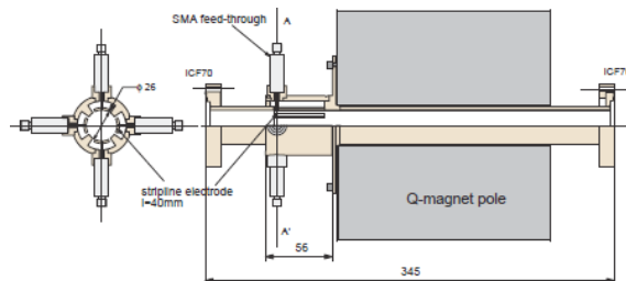
Figure 5: Stripline BPM.
