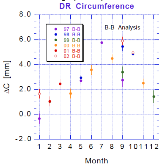
Figure 4: Change of Damping Ring Circumference, Horizontal axis indicates month on which the circumference was measured. Vertical axis is the difference between measured values and design one.
