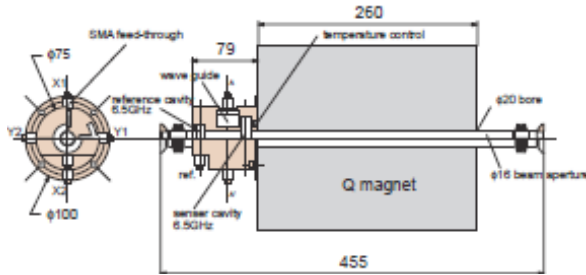
Figure 7: Cavity BPM at a Q magnet.
