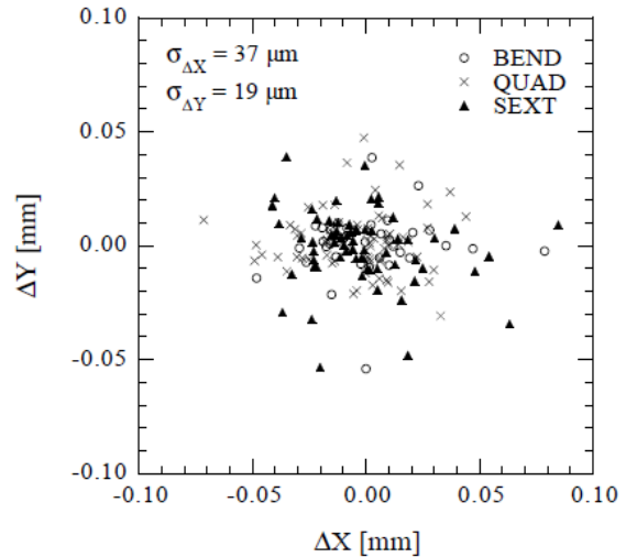
Assembly Result of Magnets on Mover Table Longitudinal Direction
