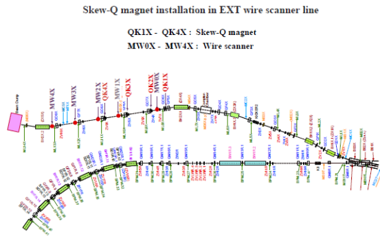
Figure 2: The layout of the extraction line.
