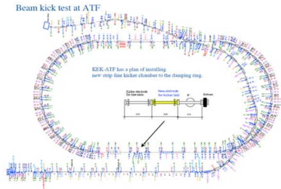
Figure 1: The Accelerator Test Facility(ATF) at KEK
