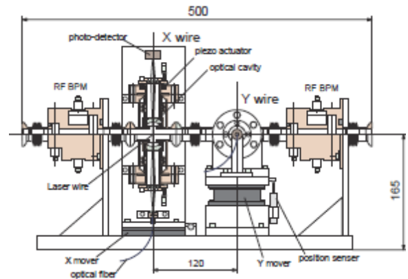
Figure 9: Laser wire scanner.
