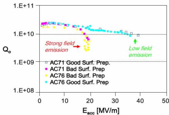
Figure 7: Examples for problems with field emission. Two cavities are shown which have been subjected to electropolishing twice. One of the tests shows strong field emission. The other tests show very good performance. So far the source of the contaminations has not been located.
