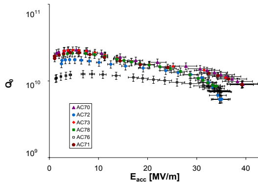
Figure 6: Several electropolished cavities yield gradients of more than 35 MV/m.
