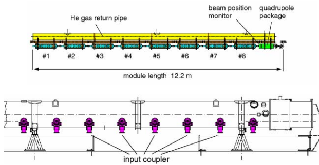
Figure 3: Layout of a TTF Accelerator module
