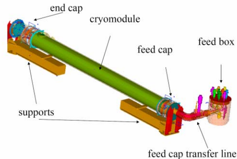
Figure 8: Layout of the module test stand. This will allow the test of accelerator modules independently of the TTF linac.
