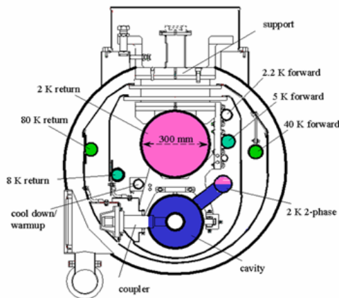
Figure 4: Cross-section of a TTF module. The last generation of cryostat design is shown.
