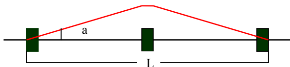
Figure 3: Timing adjustment through orbit bumps.
