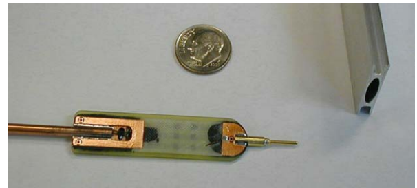
Figure 2: Assembled Hall probe and aluminum guide
