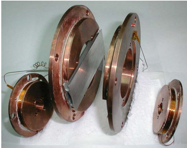
Figure 3: Calibration magnet (disassembled)
