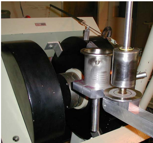
Figure 4: Cold calibration setup (Dewar disassembled)
