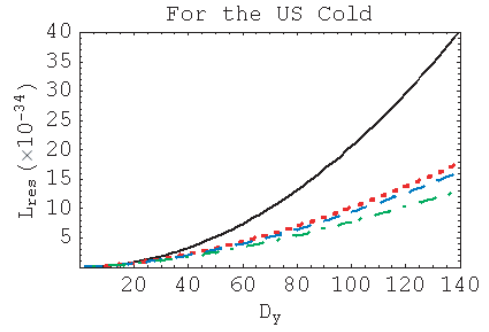
Figure 3: The resonance luminosity \mathcal{L}_{\text{res}} as a function of D_y . The dotted, dashed, and dotted-dashed curves stand for the cases where y_{r0}/\sigma_y = 1/3, 1/2 , and 1, respectively. As a comparison, the solid curve stands for the case with no modulation, i.e., \mathcal{L}_0 , or y_{r0} = 0 .
