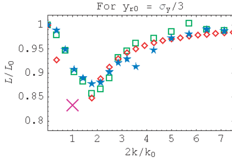
Figure 1: The \mathcal{L}/\mathcal{L}_0 as a function of 2k/k_0 . The “square” is the simulation for truncated (at \pm\sqrt{3}\sigma_z ) Gaussian distribution; the “ \star ” is the simulation for a uniform distribution; the “ \diamond ” is the result with solutions in Eqs. (10) and (11); the “ \times ” is the result with solutions in Eqs. (12) and (13).
