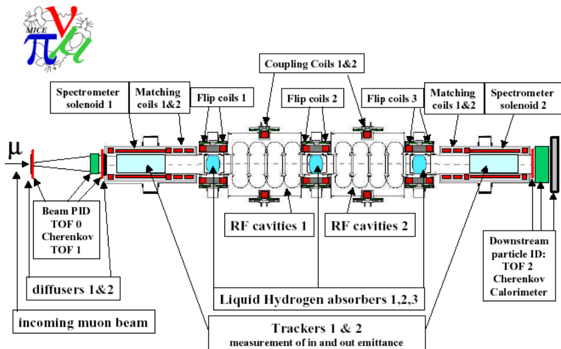
Figure 1. A Schematic Representation of MICE. (The solenoid coils are shown in dark red.)
