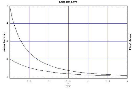
Figure 2: \gamma' as a function of normalized time t/(2\alpha) for two different initial values \gamma'_0 = 2 and \gamma'_0 = 5 .
