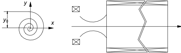
Figure 3: Entrance into solenoid. Short solenoid has focal point in front of the main one. Manipulating by polarity, location and strength of short trim pre-solenoid one can adjust the entering conditions.
