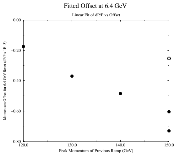
Figure 3: Momentum Offset at 6.4 GeV Reset vs. Peak of Previous Ramp for ramps with standard -300 GeV/sec downramp. Open circle for -150 GeV/sec downramp.
