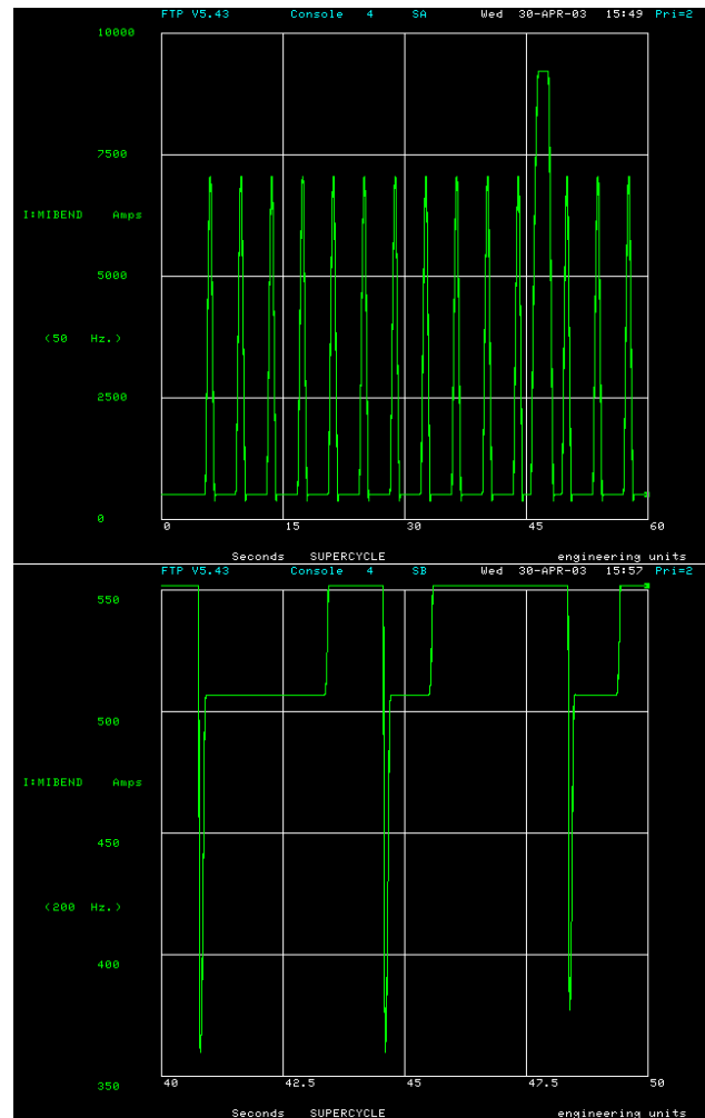
Figure 1: Main Injector Dipole magnet current vs. time in seconds in typical operation. Upper figure shows full scale with many 120 GeV ramps and a single 150 GeV ramp. Lower figure expands scale to show reset current following 120 and 150 GeV ramps. The injection porch requires a current just above 500 A.
