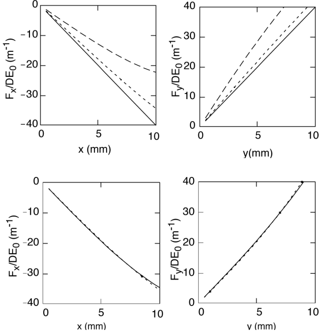
Figure 2: Force functions in a combined dipole and sextupole field. F_x at y = 0, 5, and 10 mm. F_y at x = 0, 5, and 10 mm. (upper) a_3 = 2000 . (lower) As in upper but with added decapole, a_5 = 1350000 ; off-axis forces superpose those on axis but all are now nonlinear.
