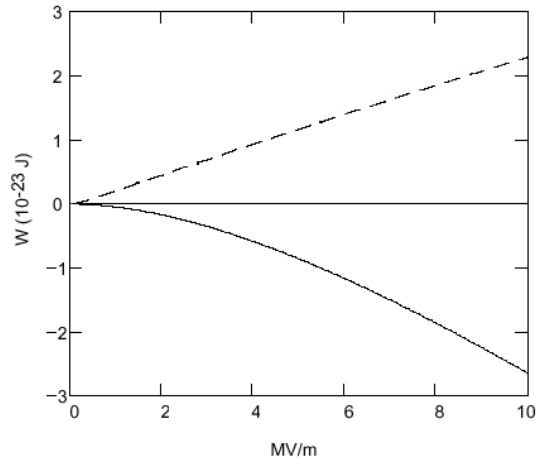
Figure 1: Potentials of methyl fluoride (CH 3 F) in the ground state (solid curve) and of deuterated ammonia (14N 2 H 3 ) in the |J,K,M\rangle=|1,1,-1\rangle state (dashed curve).
