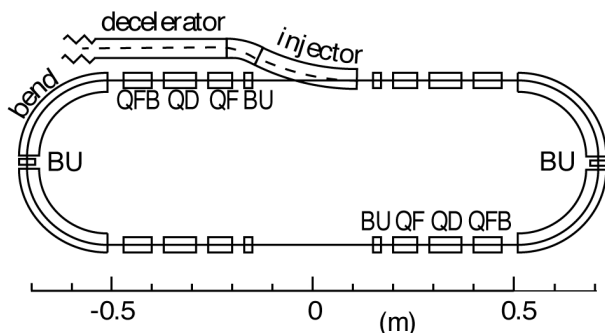
Figure 3: Layout of ring for deuterated ammonia at 90 m/s. Focusing lenses are labeled Q, and bunchers, BU.
