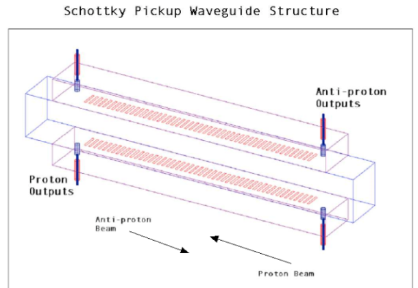
Waveguide Assembly
