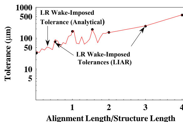
Figure 5. Alignment tolerances for H60VG3S17.
