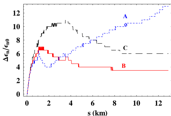
Figure 4. Simulation of \Delta\varepsilon/\varepsilon_0 , the percentage emittance growth for a single accelerating structure (A), four-fold interleaving of adjacent structures with (B) and without input HOM couplers attached (C)
