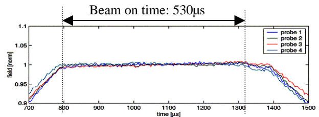
Figure 1: Signals from field probes of P2 measured during the acceleration of 530 bunches, q = 4 nC, t_b = 1 \mu\text{s} .
