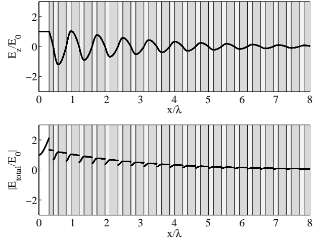
Figure 2: A typical distribution of the longitudinal electric field and the total electric field ( D_{\text{int}} = 0.3\lambda , \varepsilon^{\text{I}} = 2.1 , \varepsilon^{\text{II}} = 4 ).
