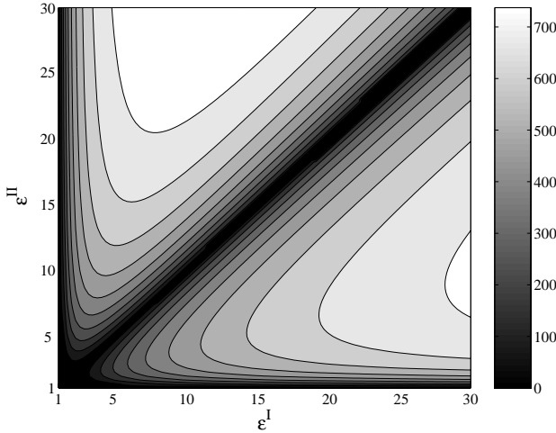
Figure 3: Contours of constant interaction impedance Z_{\text{int}}/\lambda[\Omega] as a function of (\varepsilon^{\text{I}}, \varepsilon^{\text{II}}) , with D_{\text{int}} = 0.3\lambda .
