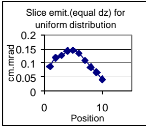
Figure 13. Slice emit.
