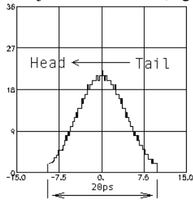
Figure 2. Laser dist.
