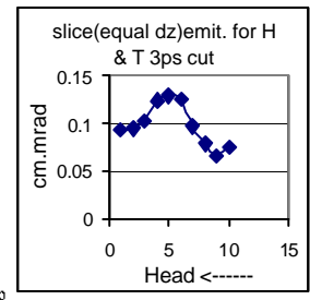
Figure 12. Slice emit.
